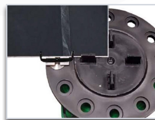
Concealed Wind Uplift Assembly 312-PPC-WUA-C*
